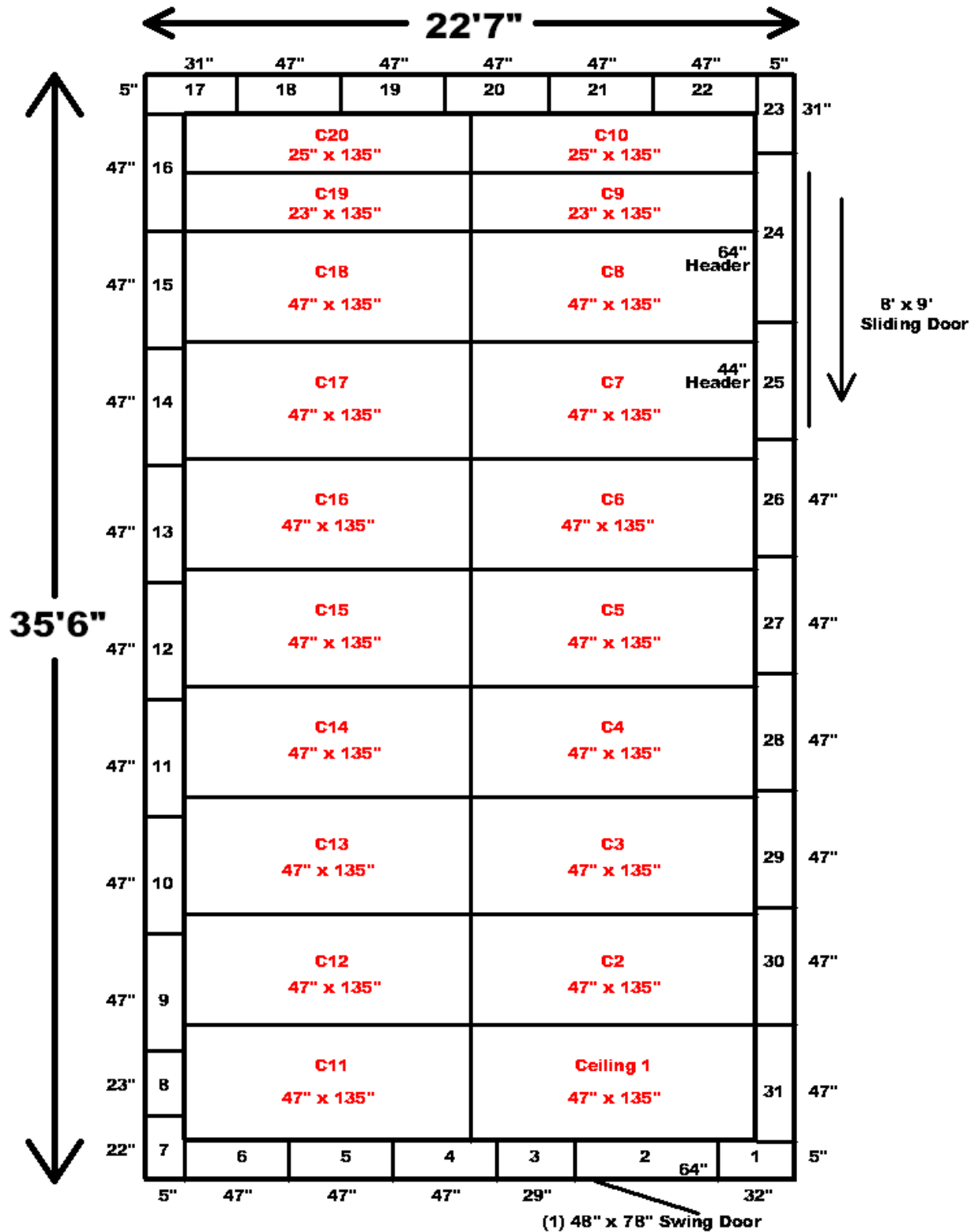
22'7" x 35'6" x 12' H Cooler Wall Panels & Ceiling Panels Diagram
