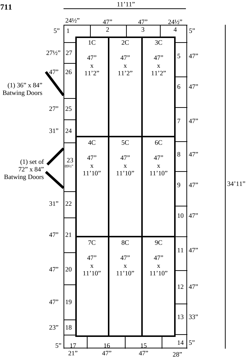
11'11" x 34'11" x 9'11" H Walk-In Cooler or Freezer Wall and Ceiling Panels Diagram
