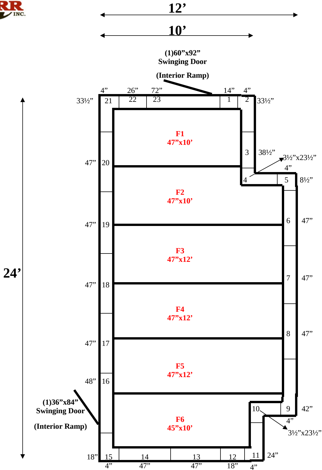
12' x 24' x 8'5" H Walk-In Freezer With Floor Wall & Floor Panels Diagram
