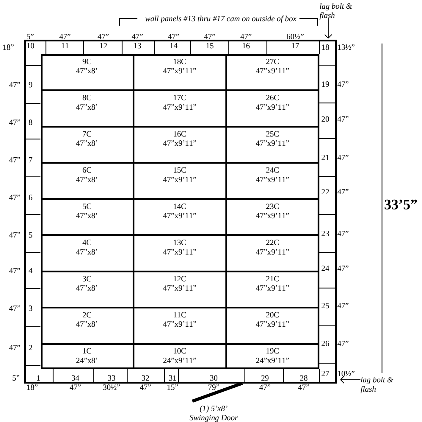
28' x 33'5" x 9'11" H Blue Walk-In Cooler or Freezer Wall and Ceiling Panels Diagram
