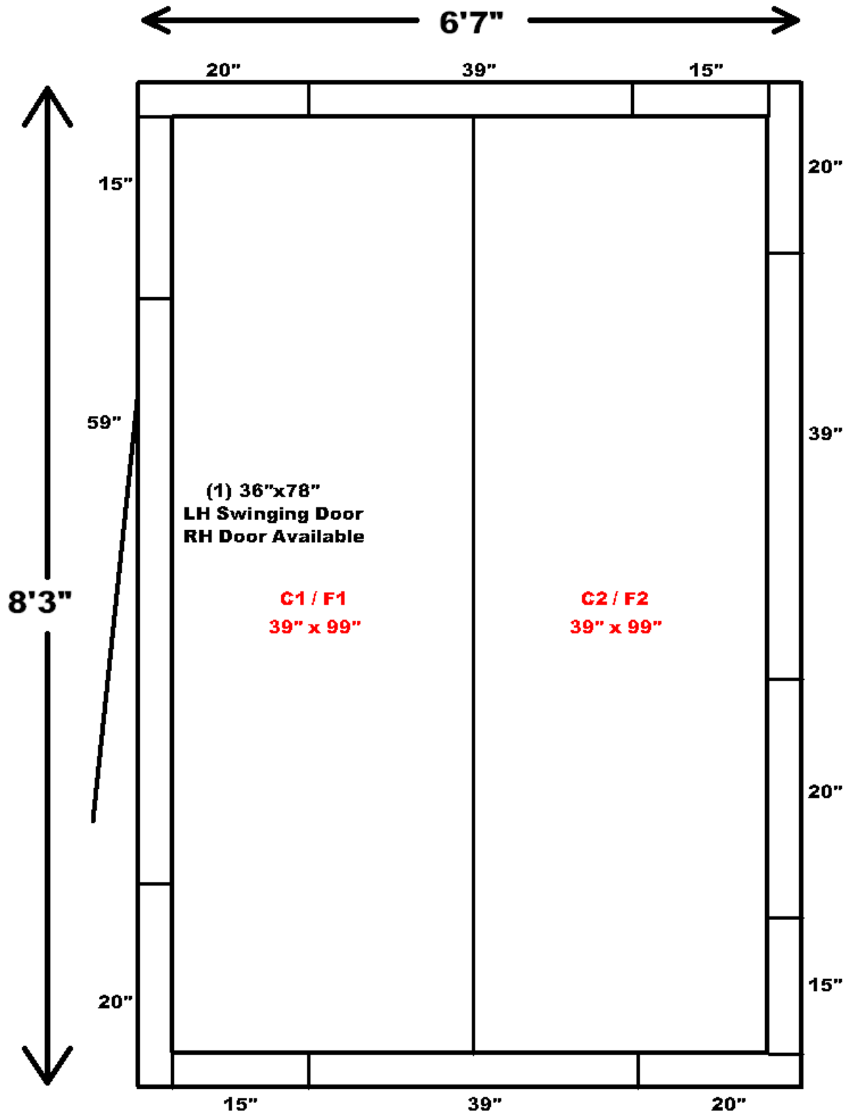
6'7" x 8'3" x 8'2" H Freezer with Floor Wall, Floor, & Ceiling Panels Diagram
