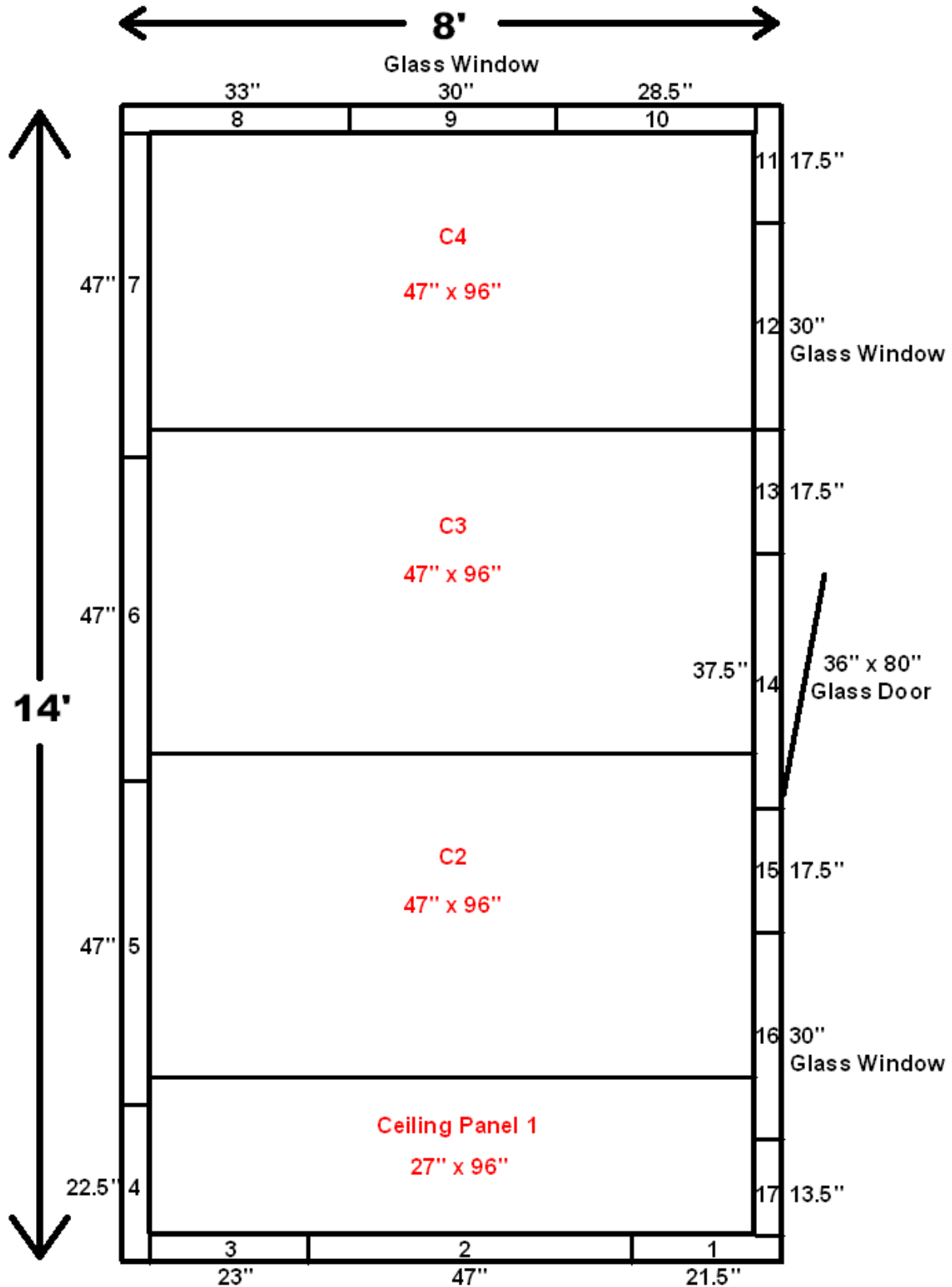
8' x 14' x 7'6" H Cooler Wall Panels & Ceiling Panels Diagram
