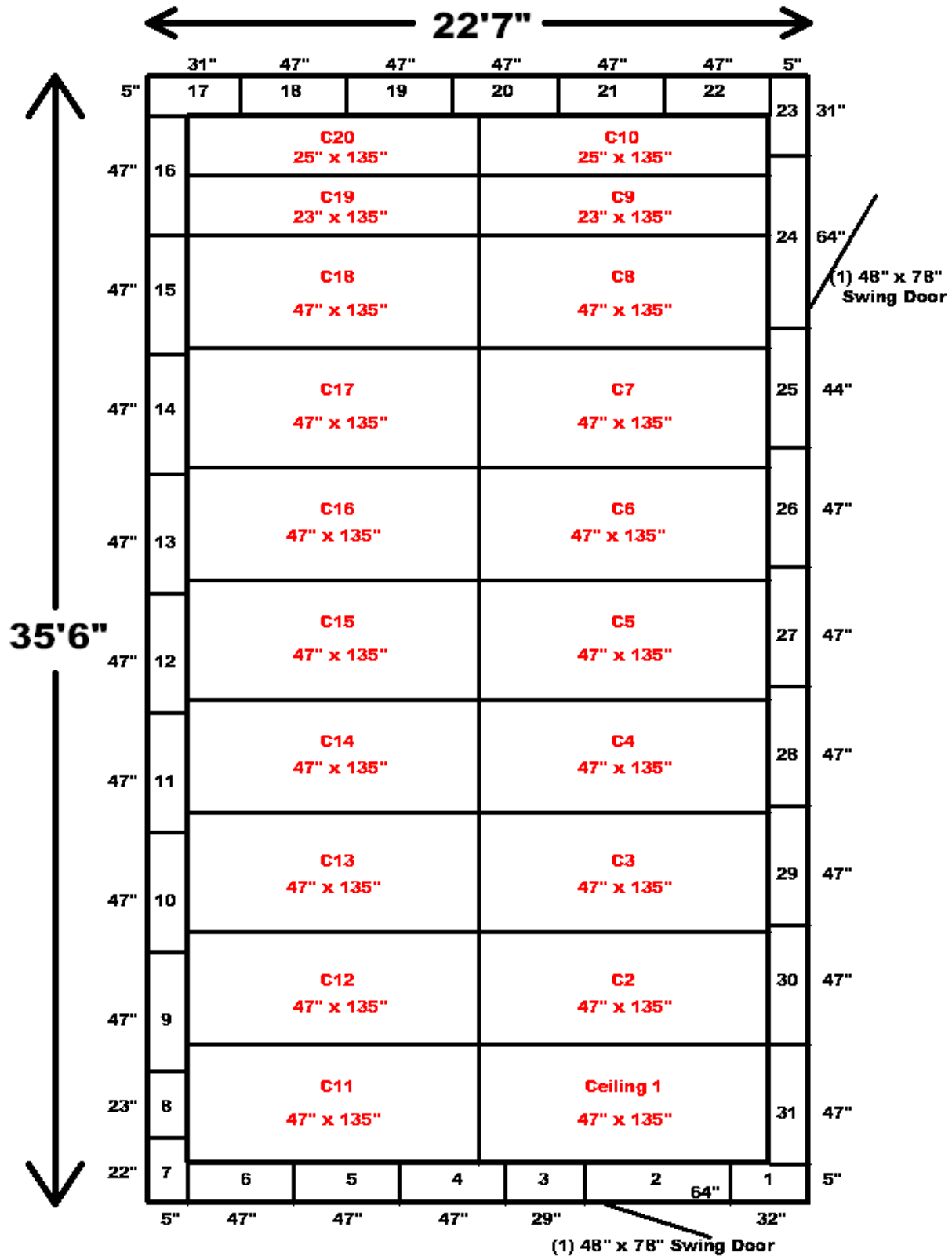
22'7" x 35'6" x 12' H Cooler Wall Panels & Ceiling Panels Diagram
