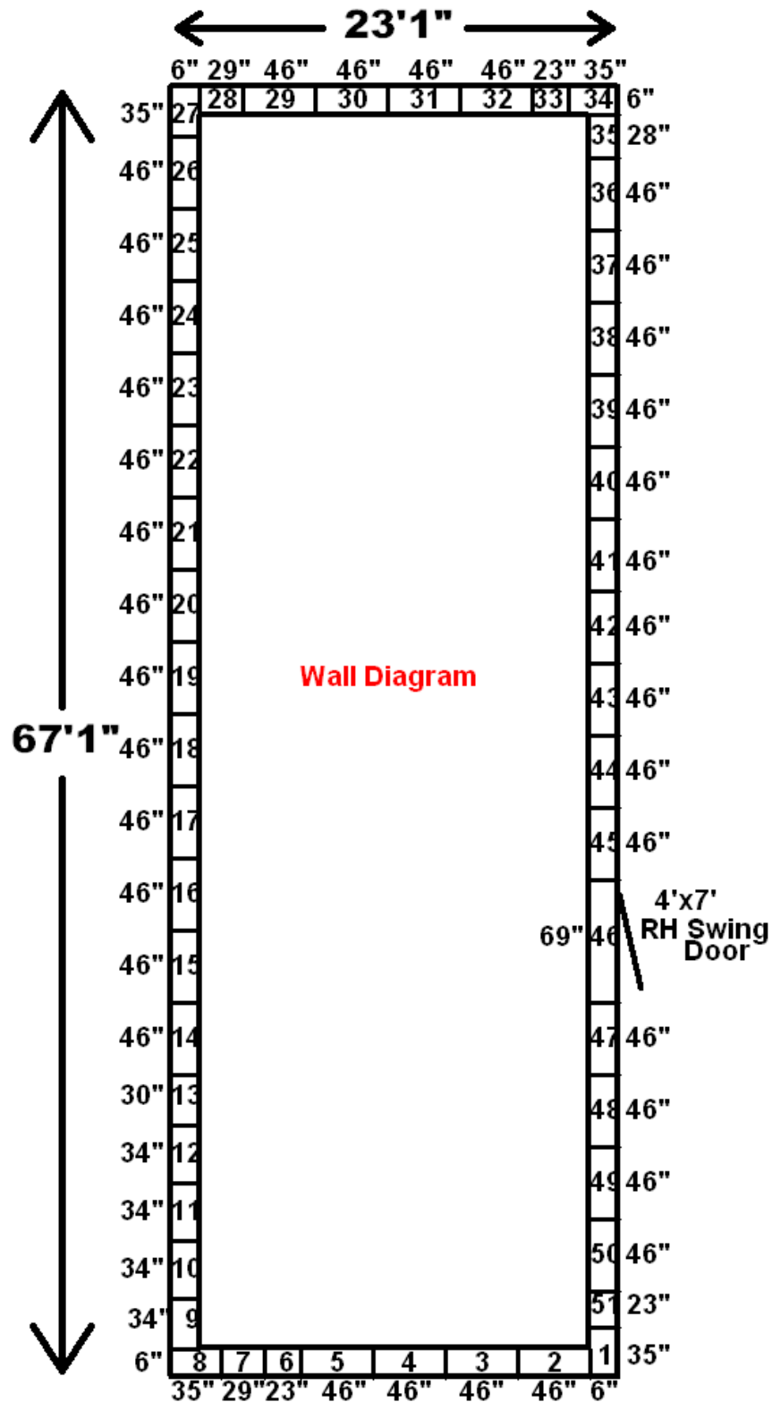
23'1" x 67'1" x 10'3" H Freezer With Floor Wall Panels Diagram
