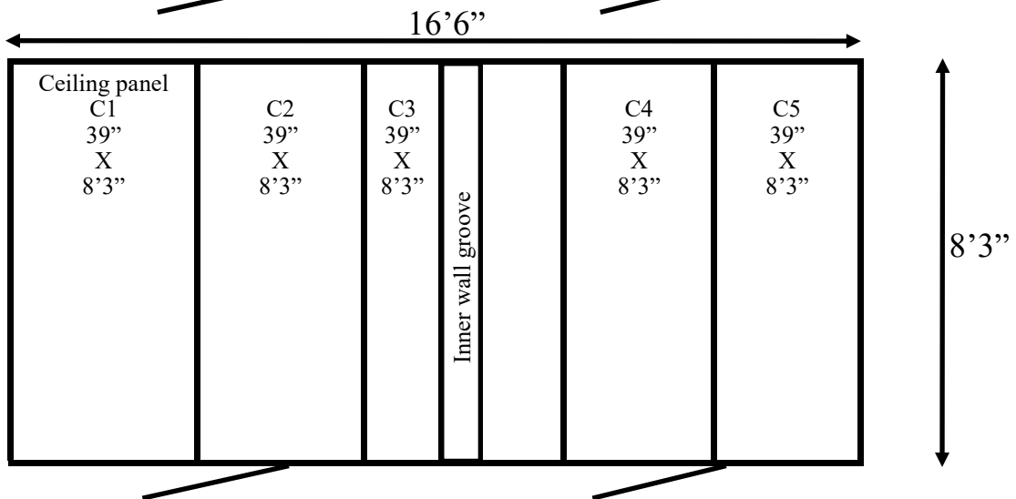
8'3" x 16'6" x 8' H Ready Ship Combo Cooler / Freezer Wall, Ceiling & Floor Panels Diagrams
