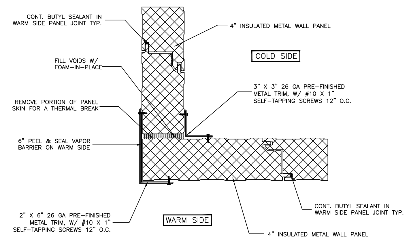
4 CORNER DETAIL A300
