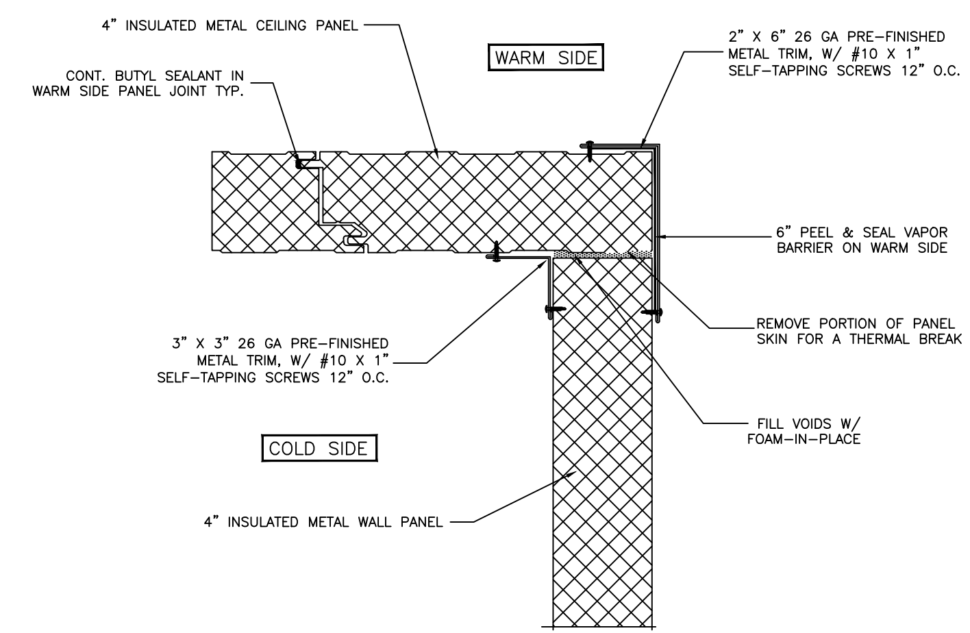
6 WALL / CEILING DETAIL A300
