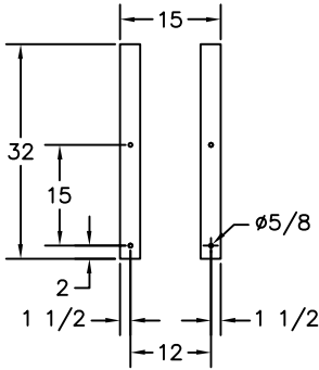
DETAIL #1 COPELAND 3 & 4 BODY COMPRESSORS
