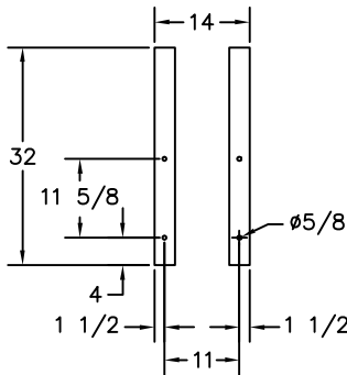
DETAIL #2 COPELAND 2 BODY COMPRESSOR
