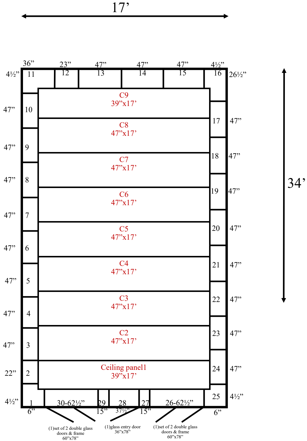
17' x 34' x 10' H Cooler with Glass Doors Wall & Ceiling Panels Diagram
