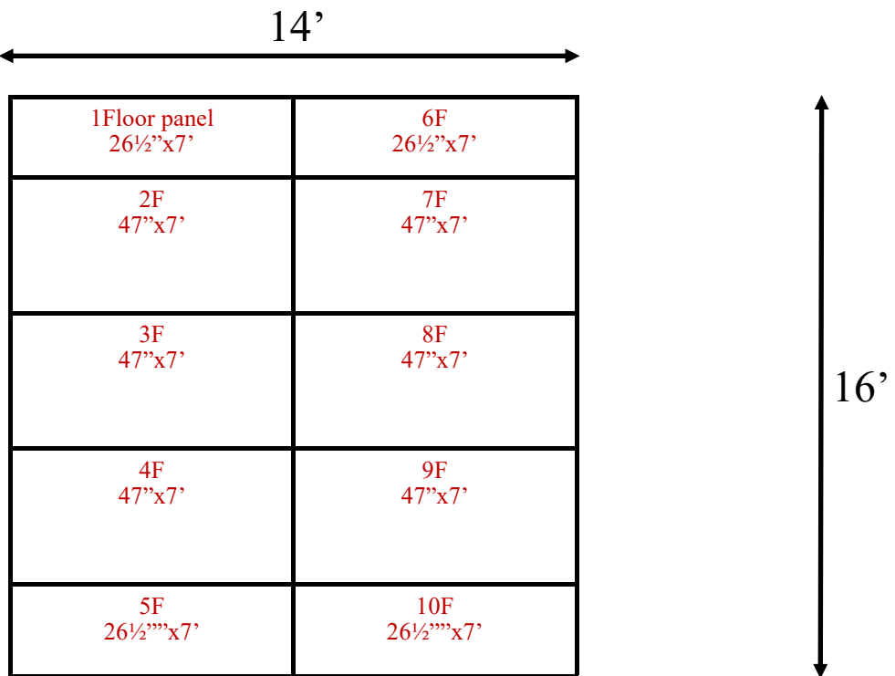
14' x 16' x 8' H Freezer with Floor Wall, Ceiling & Floor Panels Diagram
