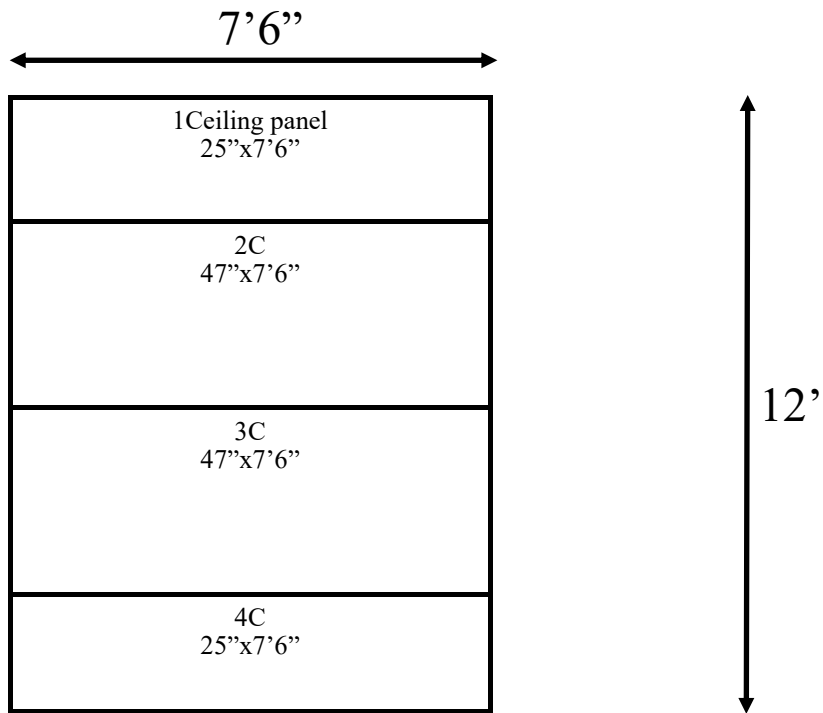
7'6" x 12' x 8' H Cooler / Freezer Combination Wall & Ceiling Panels Diagram
