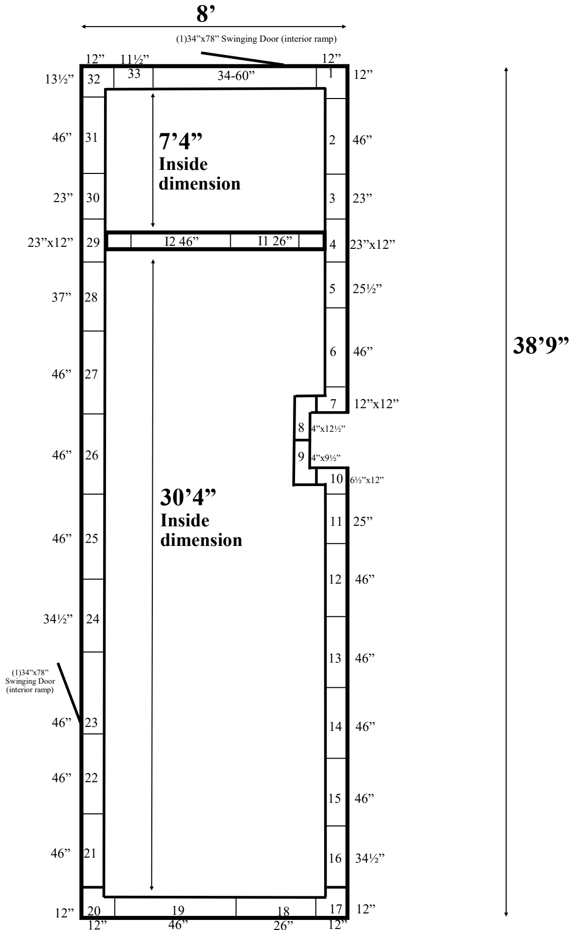
8' x 38'9" x 8'6" H Combination Cooler / Freezer Wall, Ceiling & Floor Panels Diagram
