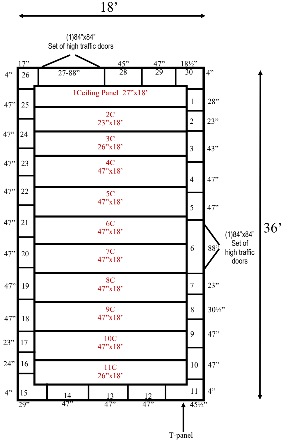
18' x 36' x 9'6" H Cooler Wall & Ceiling Panels Diagram
