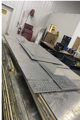
14' x 16' x 10'6" H Freezer with Floor
