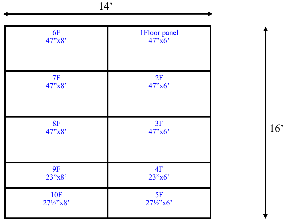
14' x 16' x 10'6" H Freezer with Floor Wall, Ceiling & Floor Panels Diagram
