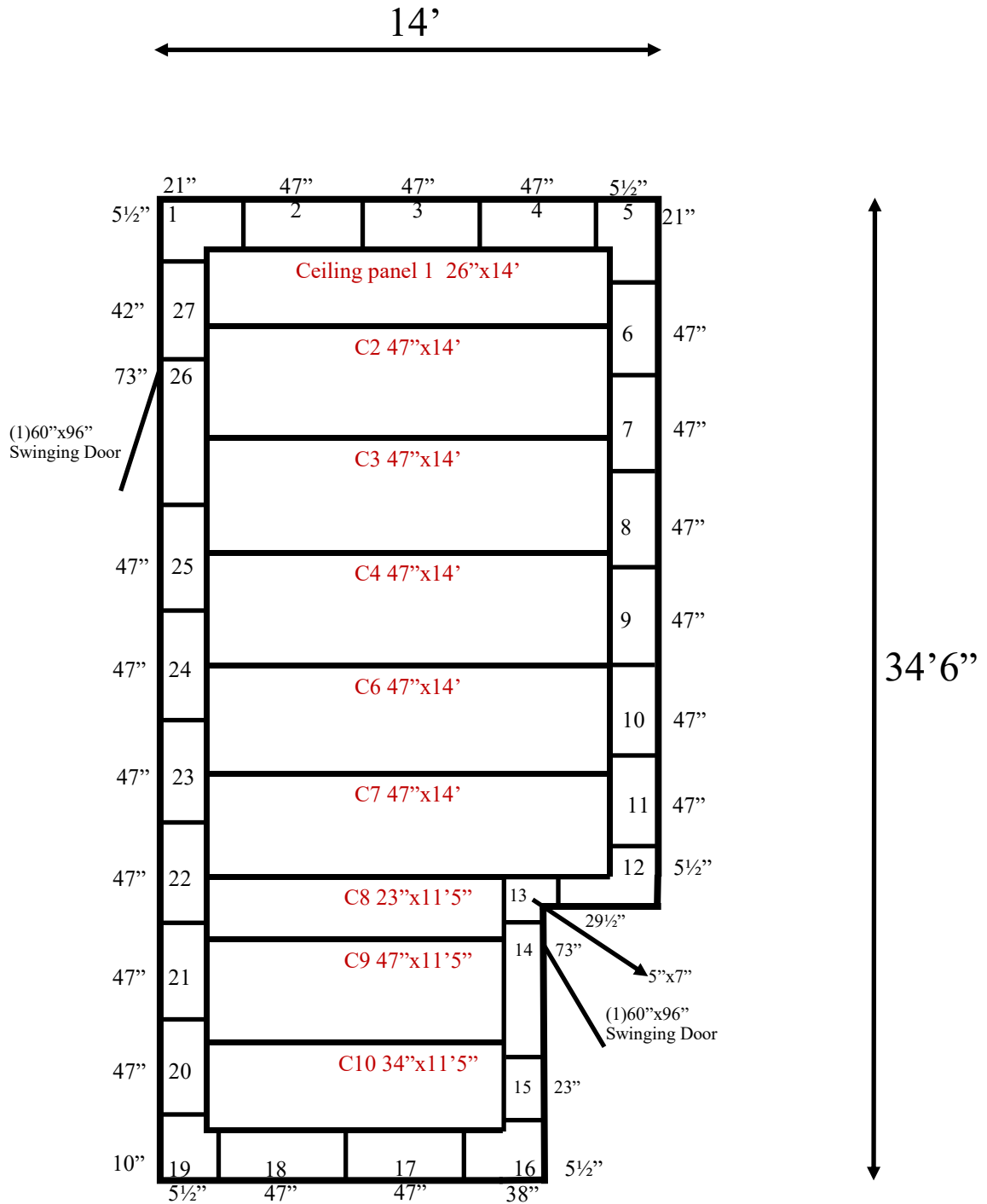
14' x 34'6" x 10' H Cooler Wall & Ceiling Panels Diagram
