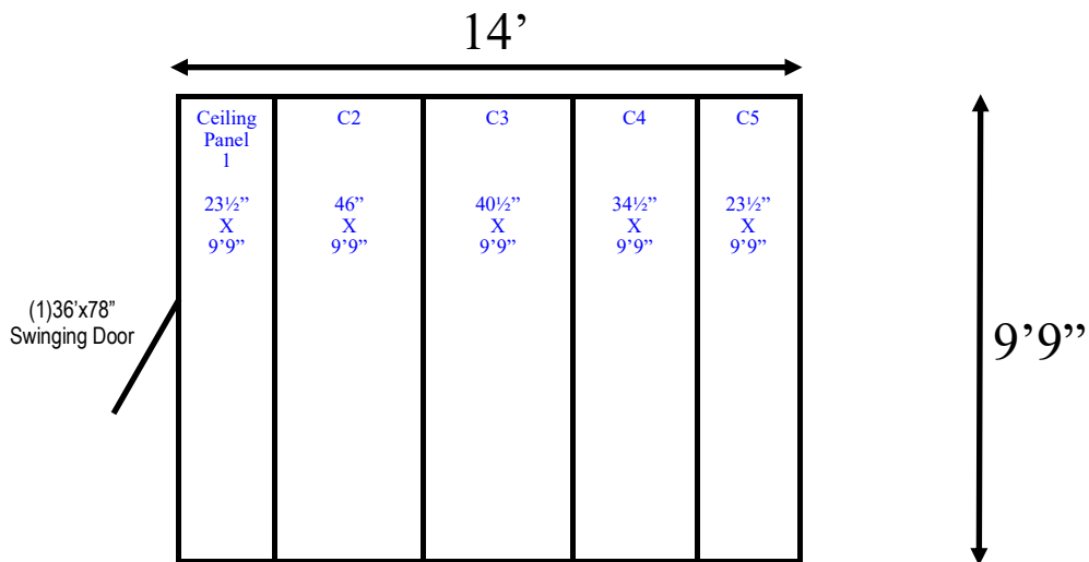
9'9" x 14' x 8' H Combo Cooler / Freezer Wall, Ceiling & Floor Panel Diagrams
