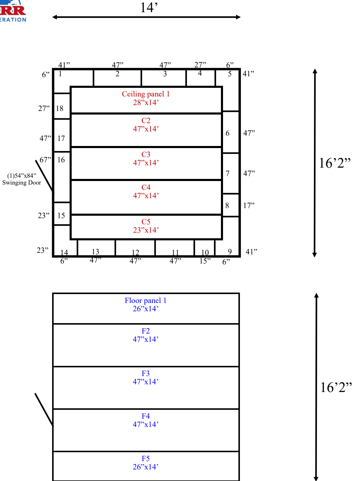
14' x 16'2" x 9'2" H Freezer with Floor Wall, Ceiling & Floor Panels Diagram
