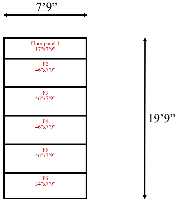
7'9" x 19'9" x 8'7"H Cooler with Floor Wall, Ceiling & Floor Panel Diagrams
