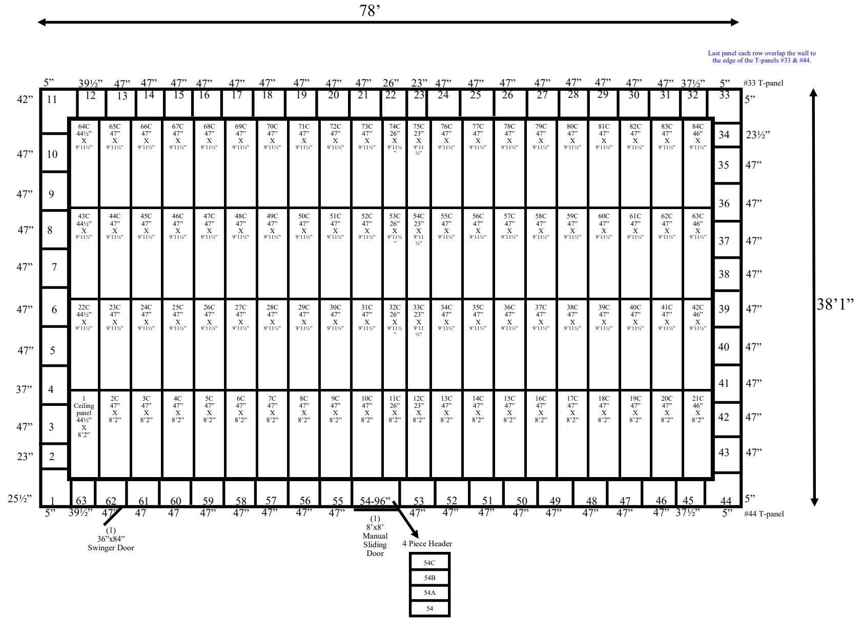
38'1" x 78' x 22' H Cooler Wall & Ceiling Panels Diagram
