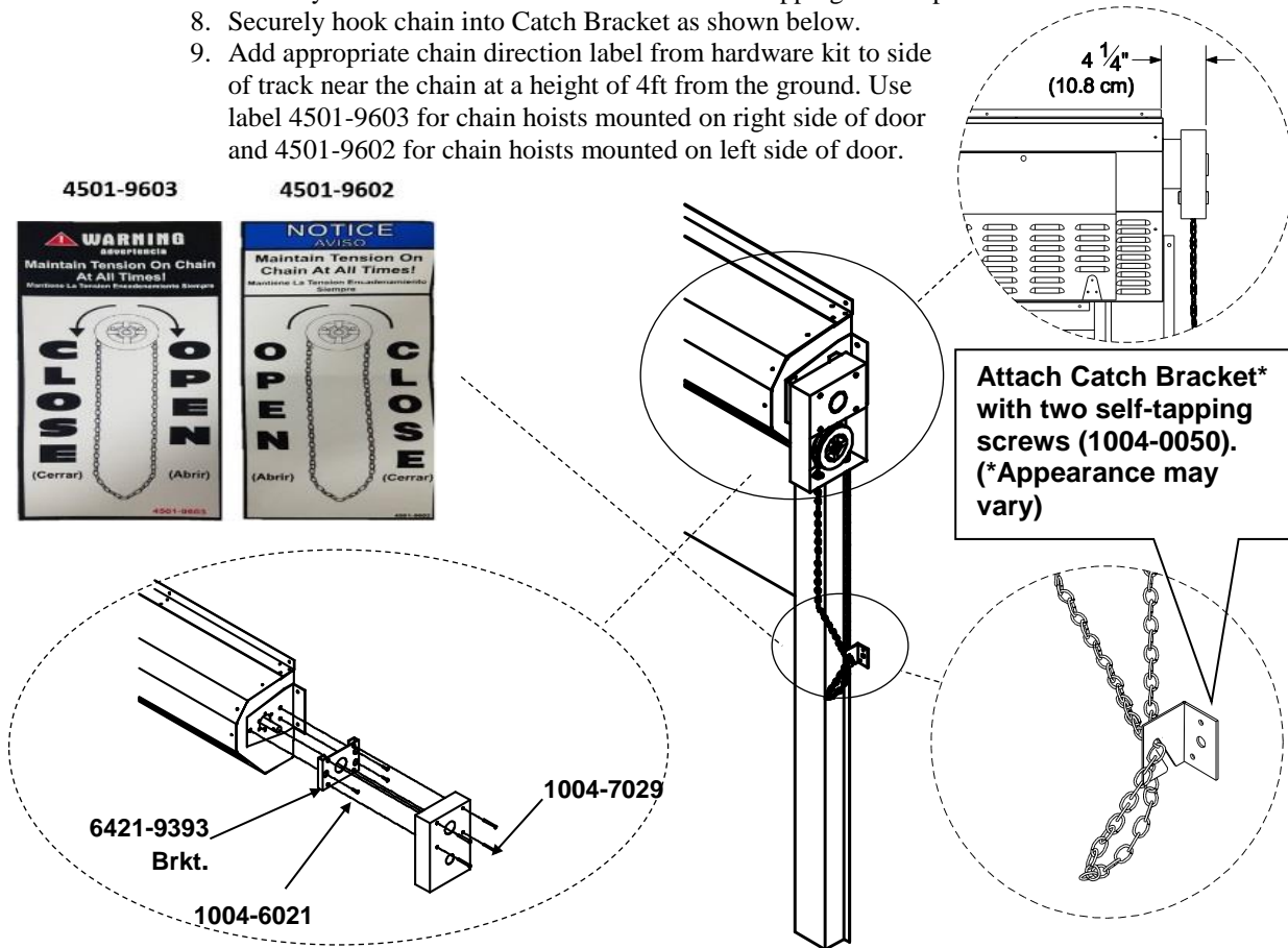
Diagram 17B Chain Hoist
