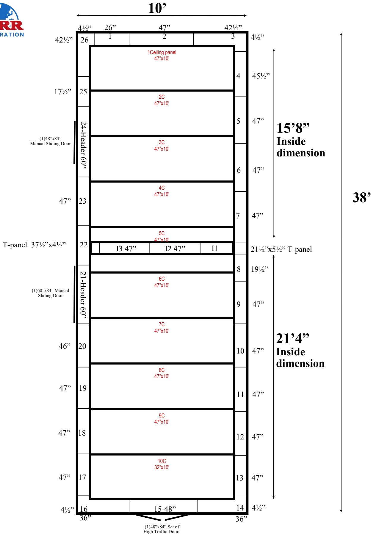
10' x 38' x 10'7" H Cooler / Freezer Combination Wall & Ceiling Panels Diagram
