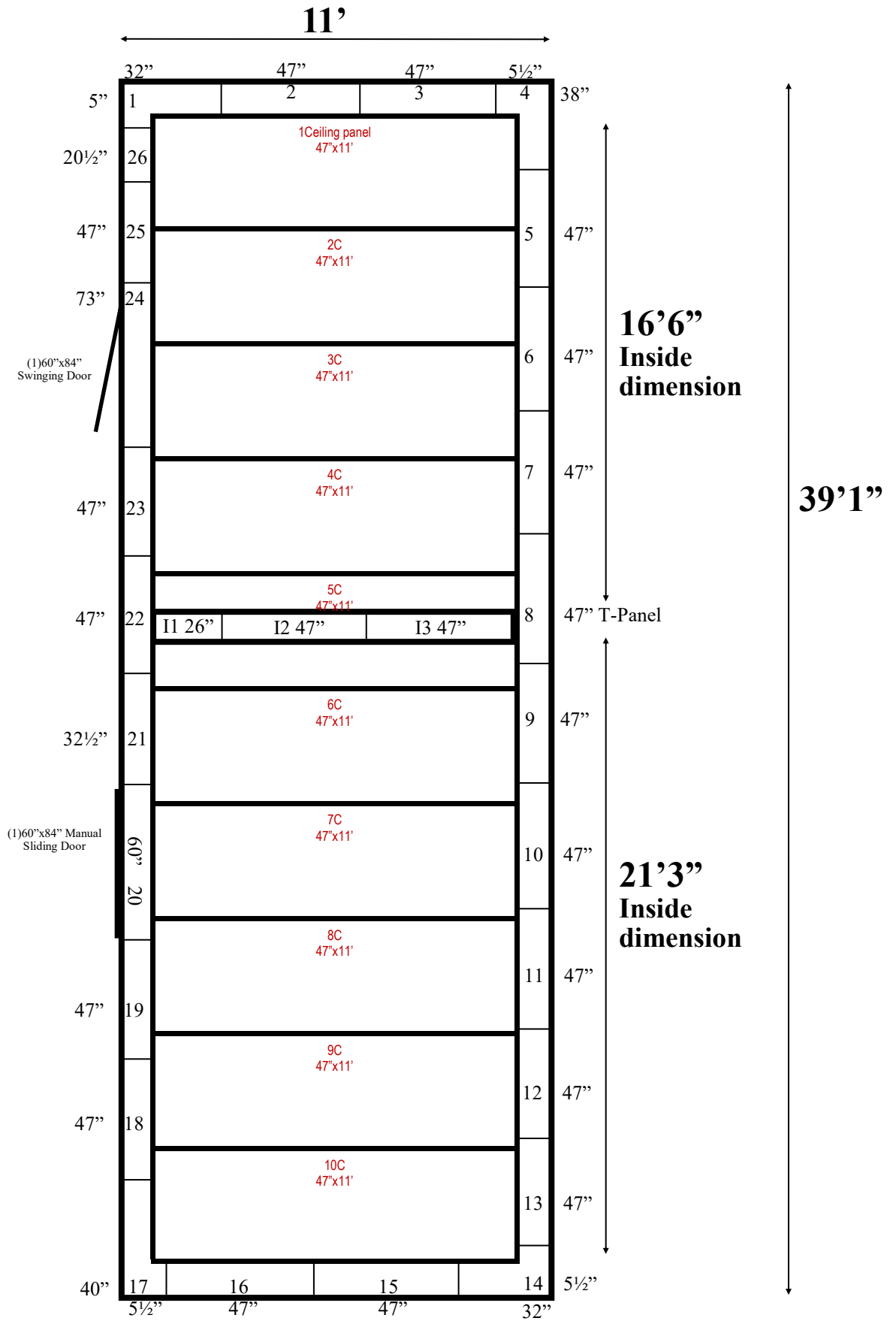
11' x 39'1" x 10' H Combination Cooler / Freezer Wall & Ceiling Panels Diagram
