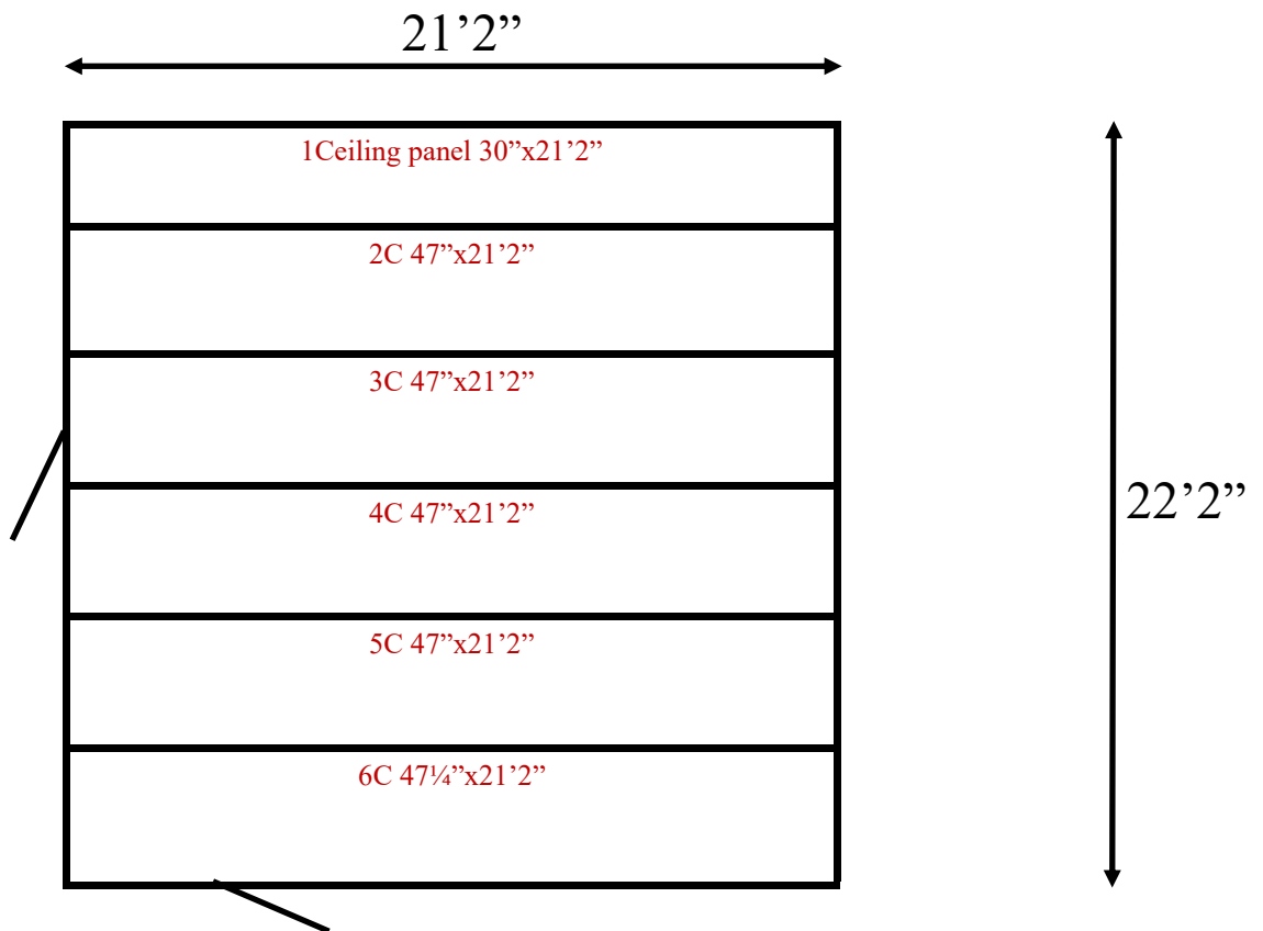
21'2" x 22'2" x 8'10" H Freezer with Floor Wall, Ceiling & Floor Panel Diagrams
