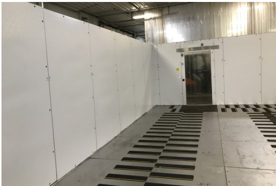
24' x 35'7" x 8'6" H Freezer with Floor
