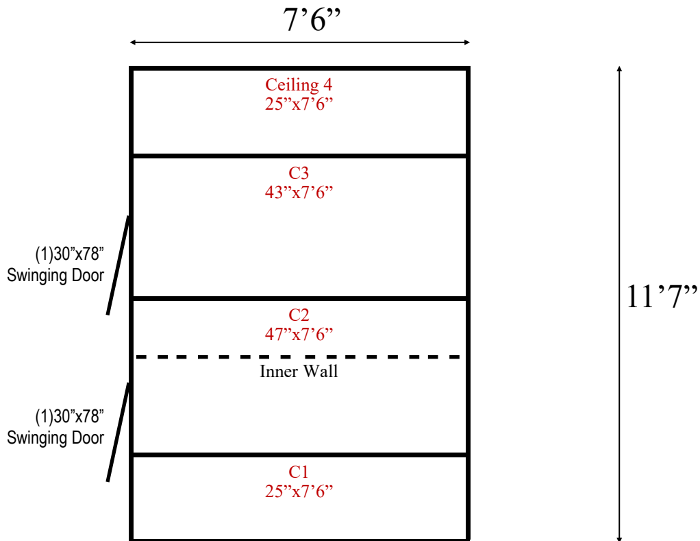
7'6" x 11'7" x 8' H Cooler/Freezer Combination Wall & Ceiling Panel Diagrams
