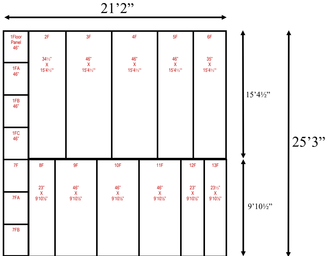
21'2" x 25'3" x 10' H Combination Cooler / Freezer With Floor Wall, Ceiling & Floor Panels Diagram
