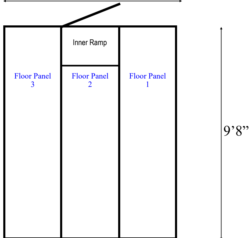
7'9" x 9'8" x 9' H Freezer With Floor Wall, Ceiling & Floor Panels Diagram
