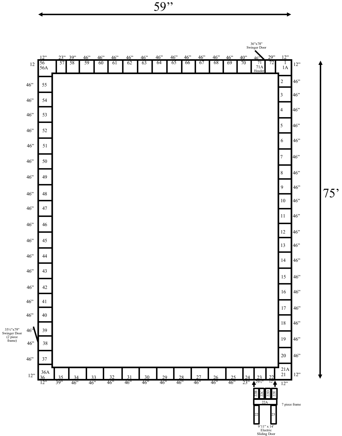
59' x 75' x 27' H Cooler or Freezer Wall Panels Diagram
