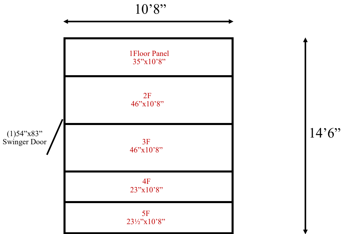
10'8" x 14'6" x 8'6" H Cooler with Floor Wall, Ceiling & Floor Panels Diagram
