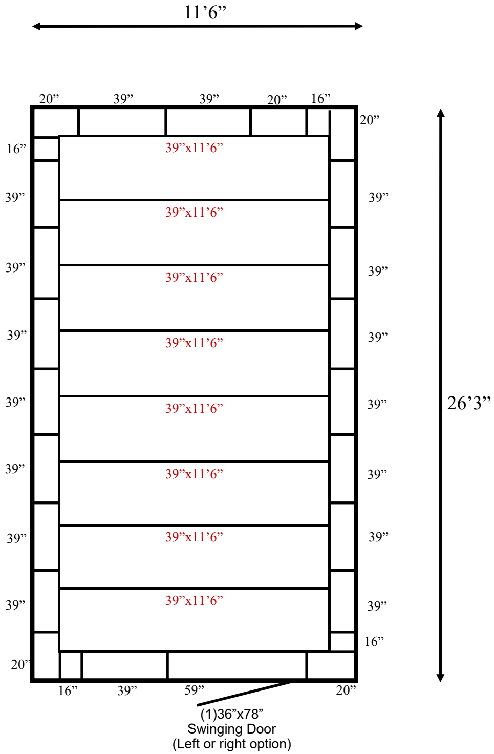
11'6" x 26'3" x 8' H Barr Ready Ship Cooler Wall & Ceiling Panels Diagram
