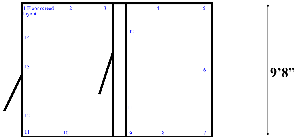
9'8" x 13'6" x 7'6" H Cooler / Freezer Combination Wall, Ceiling & Floor Screed Panel Diagrams
