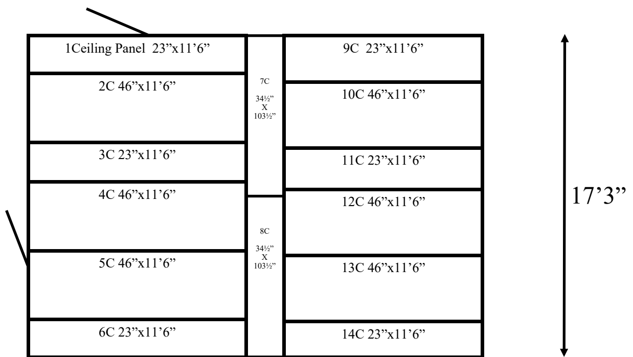
17'3" x 25'10" x 9'1" H (11' H with beam) Cooler or Freezer Wall & Ceiling Panels Diagram
