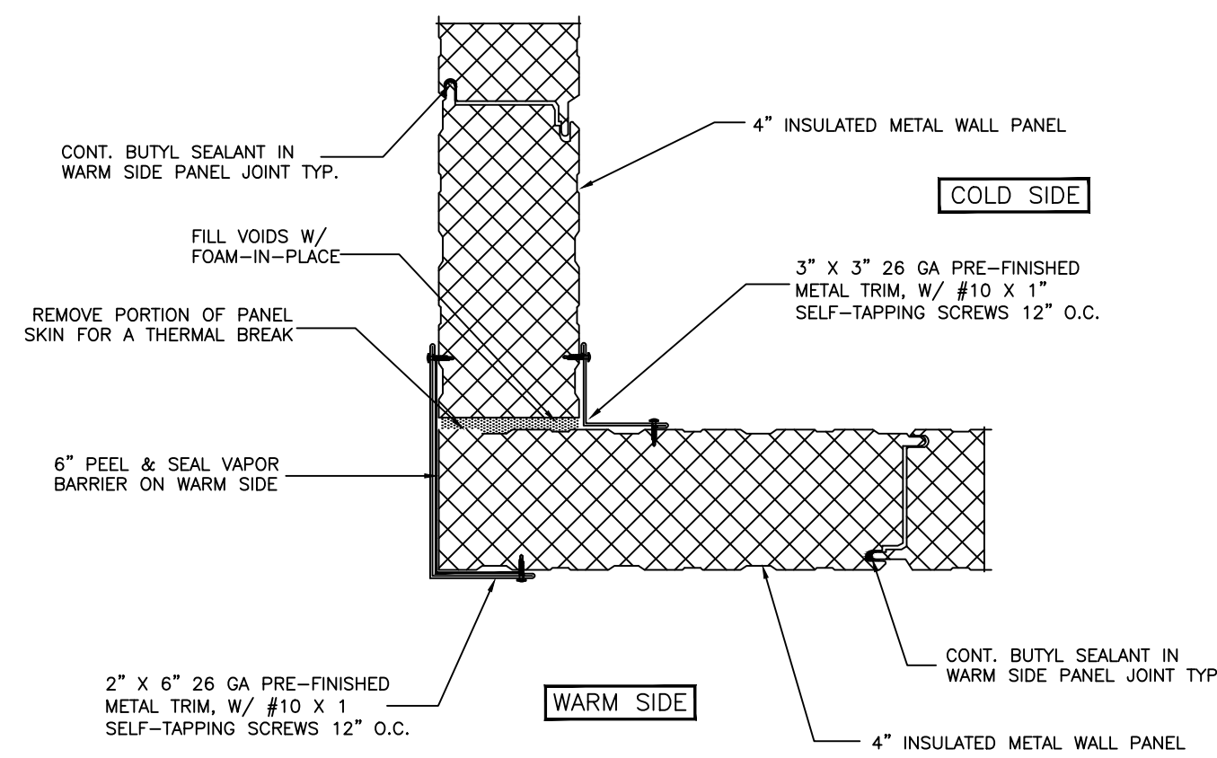
5 CORNER DETAIL A300
