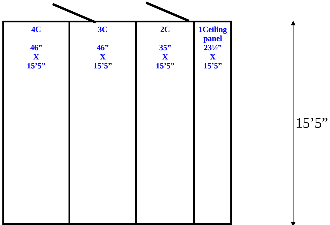
12'7" x 15'5" x 8'6" H Walk-In Combination Cooler / Freezer with Floor Wall, Ceiling & Floor Panels Diagram
