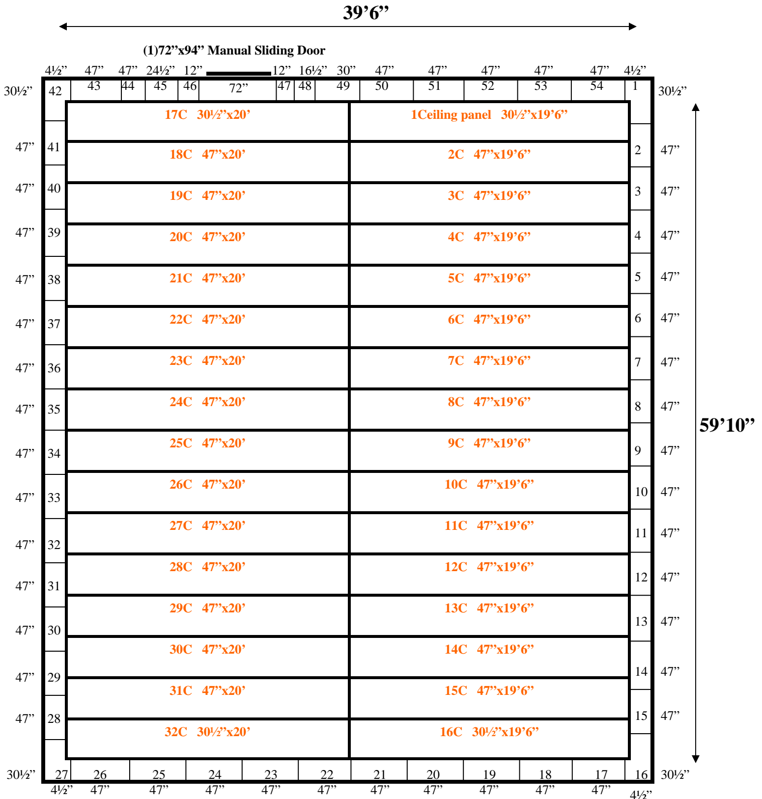
39'6" x 59'10" x 10'7" H Freezer with Floor Wall & Ceiling Panels Diagram
