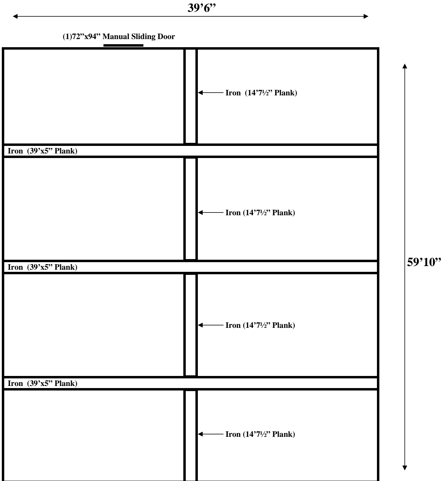
39'6" x 59'10" x 10'7" H Freezer with Floor Ceiling Support (on top of box)
