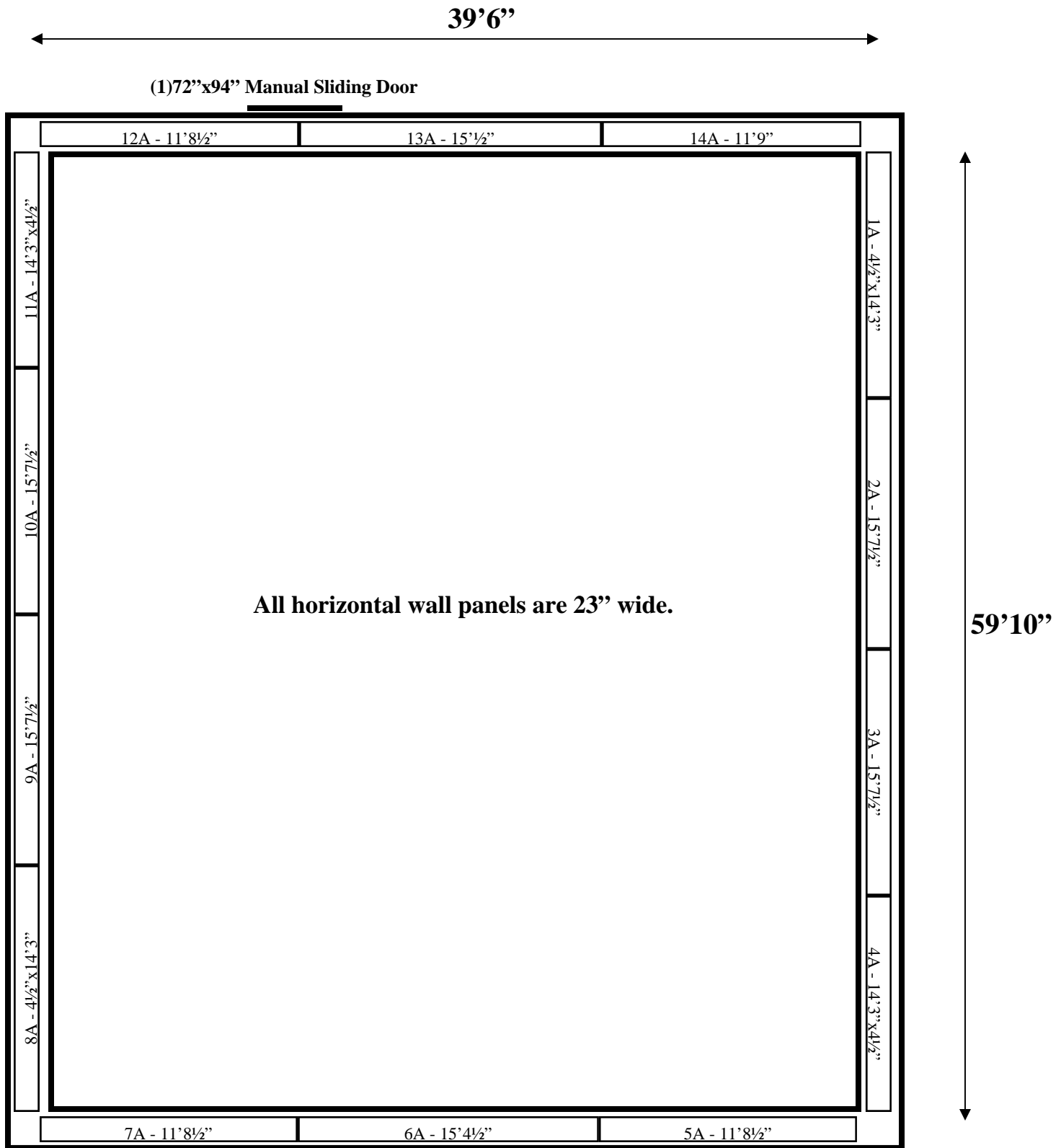
39'6" x 59'10" x 10'7" H Freezer with Floor Horizontal Wall Panels Diagram
