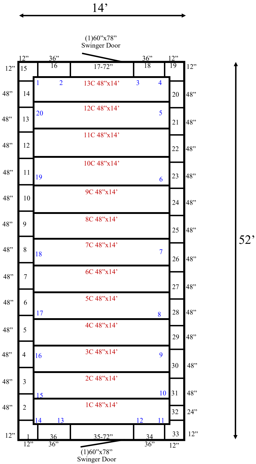
14' x 52' x 8'4" H Cooler or Freezer Wall & Ceiling Panels Diagram
