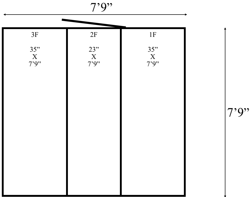
7'9" x 7'9" x 8'8" H Freezer With Floor Wall, Ceiling & Floor Panels Diagram
