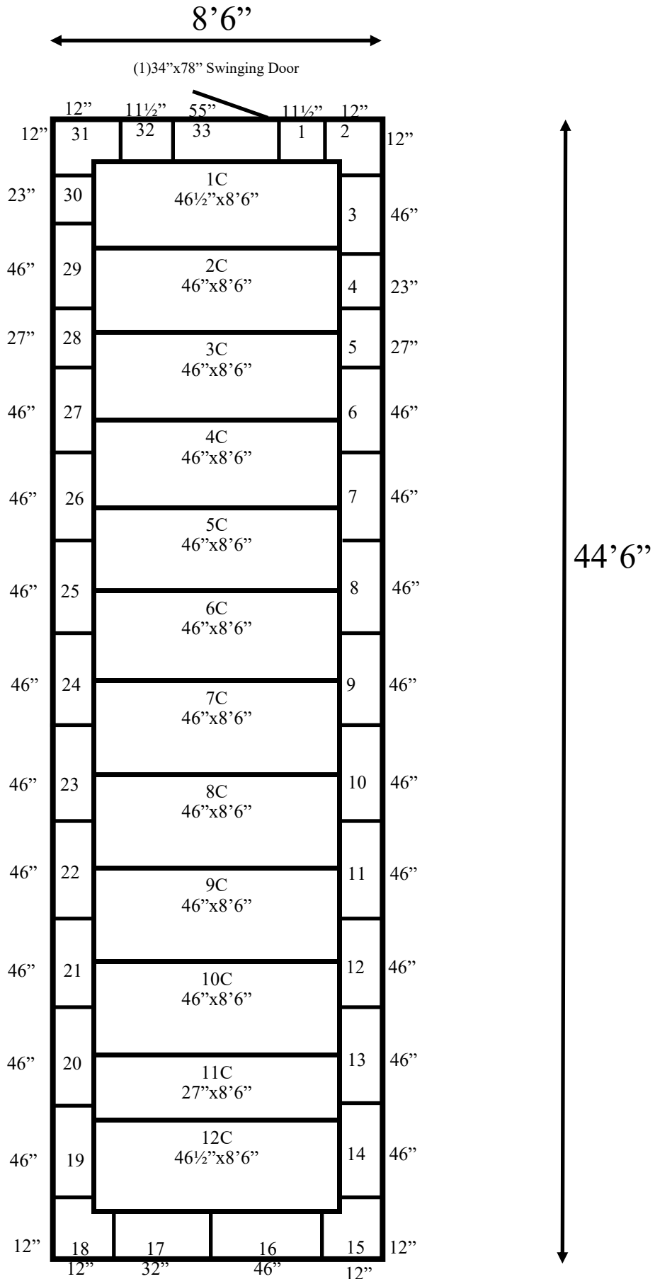
8'6" x 44'6" x 7'2" H Cooler or Freezer Wall & Ceiling Panels Diagram
