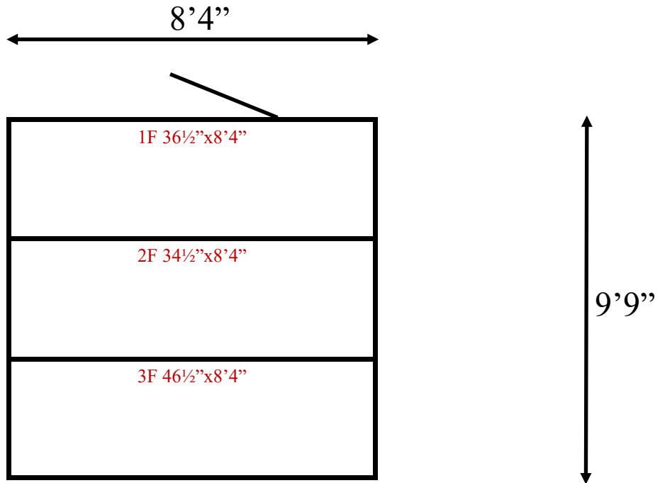
8'4" x 9'9" x 8'7" H Freezer With Floor Wall, Ceiling & Floor Panels Diagram
