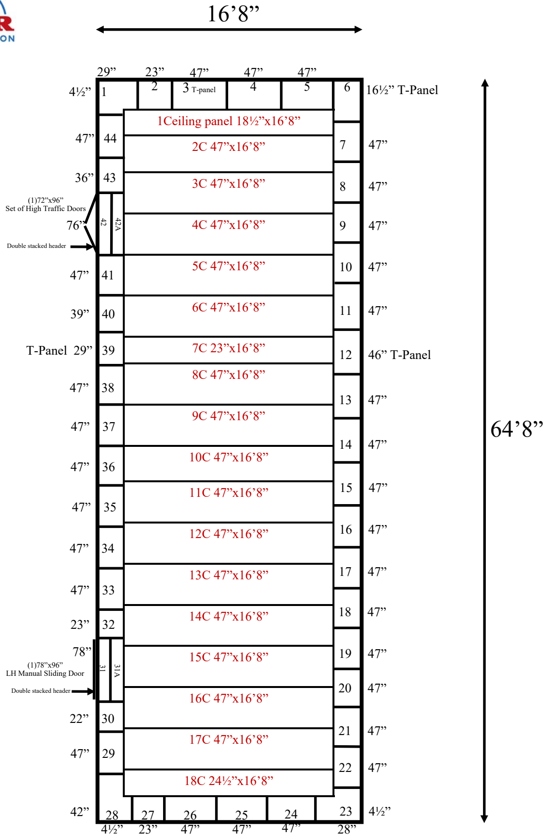
16'8" x 64'8" x 15'6" H Cooler or Freezer Wall & Ceiling Panels Diagram
