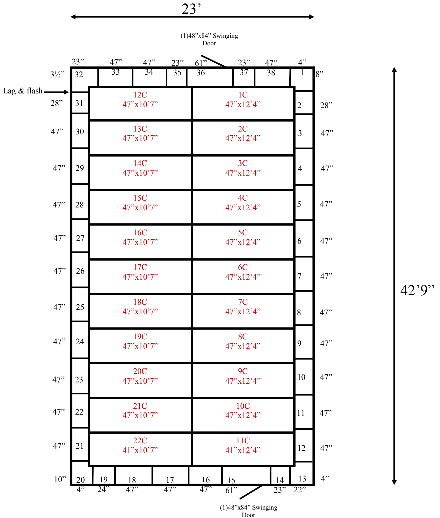
23' x 42'9" x 11' H Cooler or Freezer Wall & Ceiling Panels Diagram
