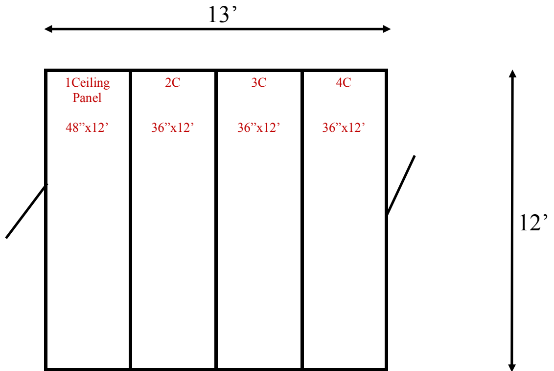
12' x 13' x 8'4''H Combination Cooler / Freezer Wall & Ceiling Panels Diagram
