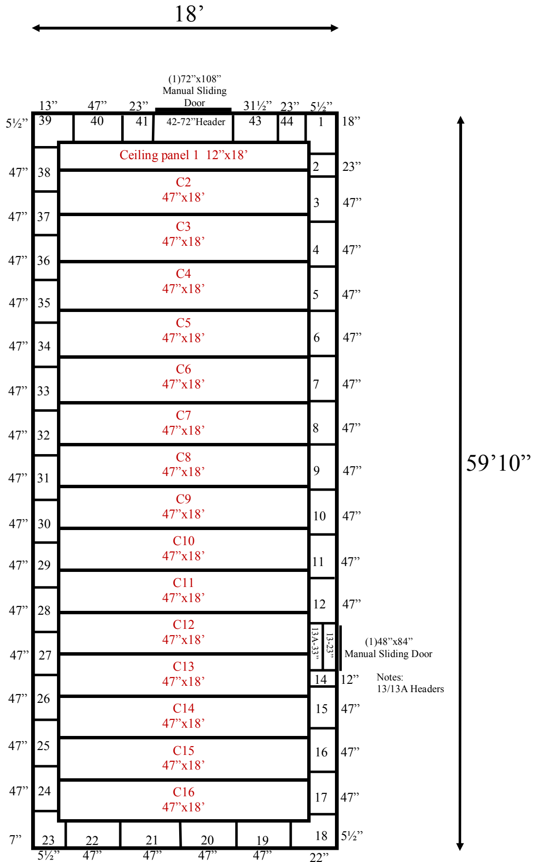
18' x 59'10" x 12' H Cooler or Freezer Wall & Ceiling Panels Diagram
