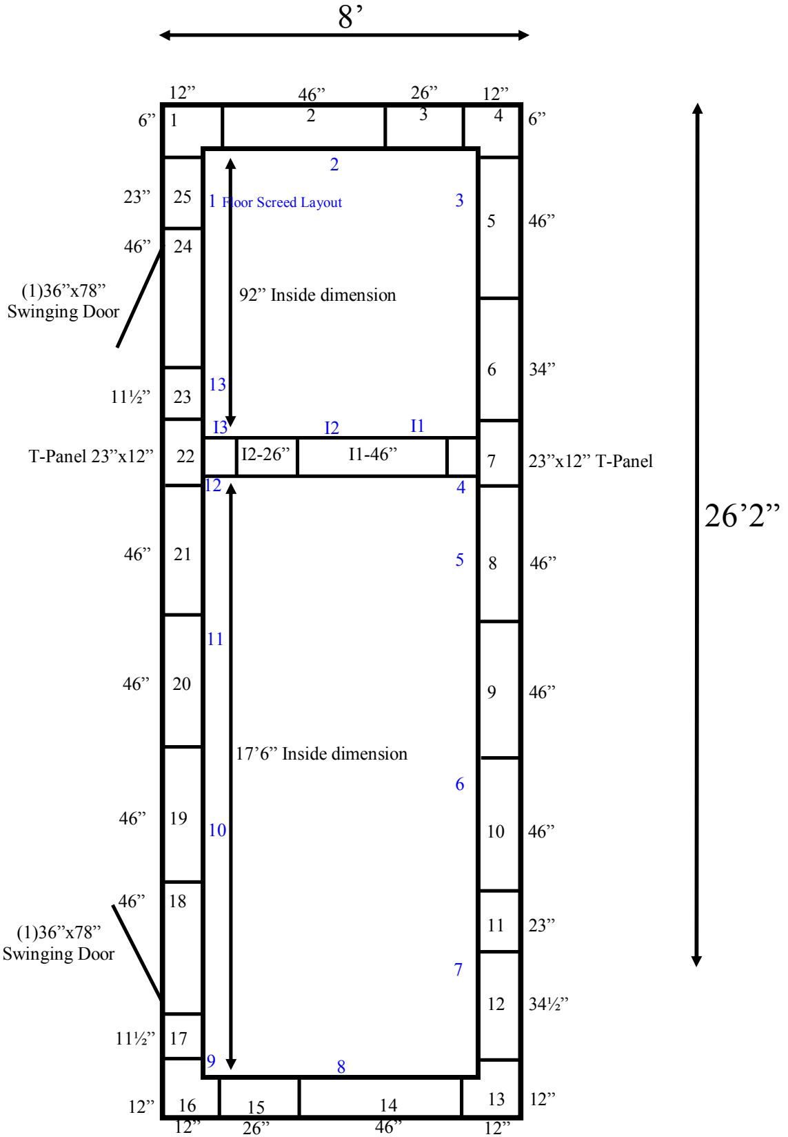
8' x 26'2" x 8'4" H Cooler /Freezer Combination Wall Panels Diagram
