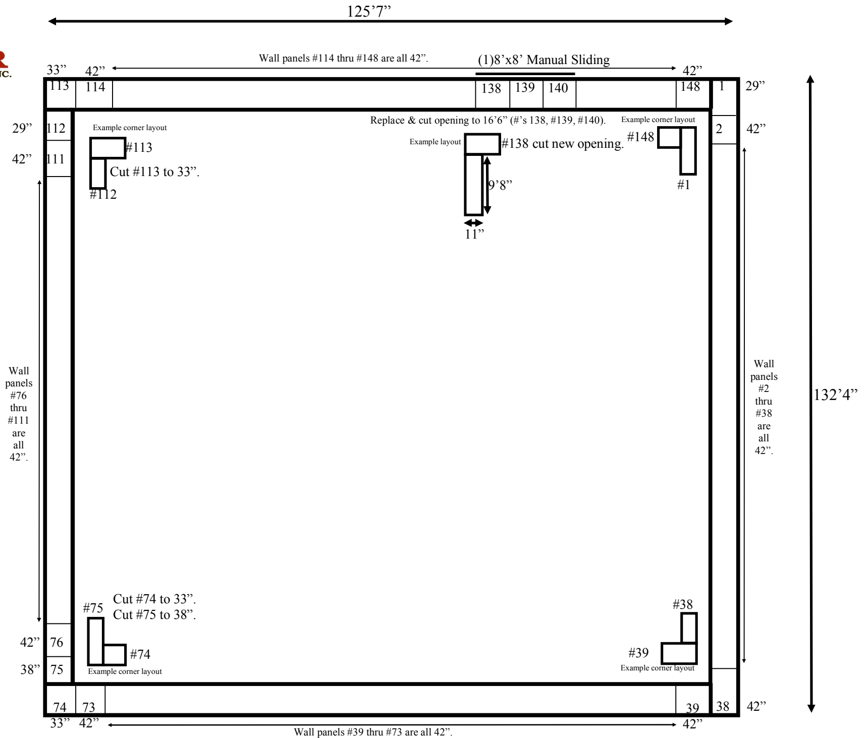
125'7" x 132'4" x 25' Drive-In Cooler or Freezer Wall Panels Diagram
