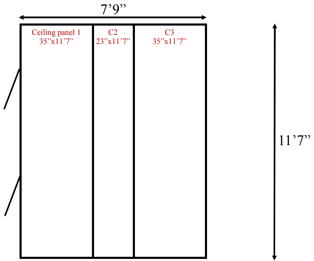
7'9" x 11'7" x 8'6" H Cooler / Freezer Combination Wall & Ceiling Panel Diagrams
