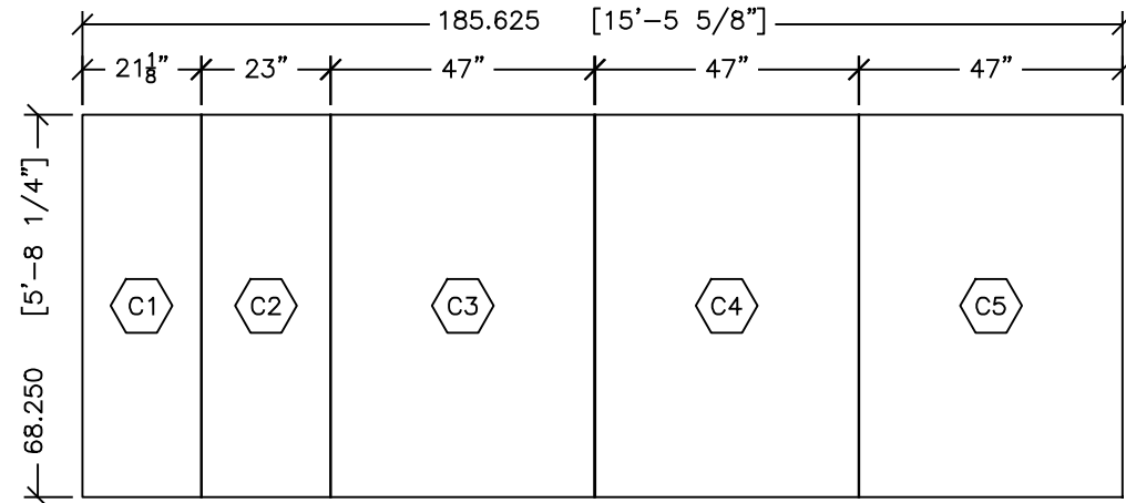
4" LAG CEILING TOP VIEW
