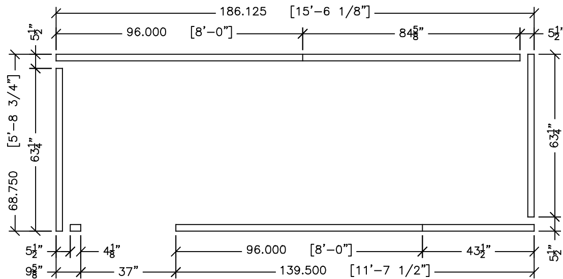
2 1/2" WOOD SCREED TOP VIEW
